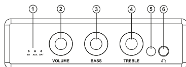
Fig. 1. Control panel
