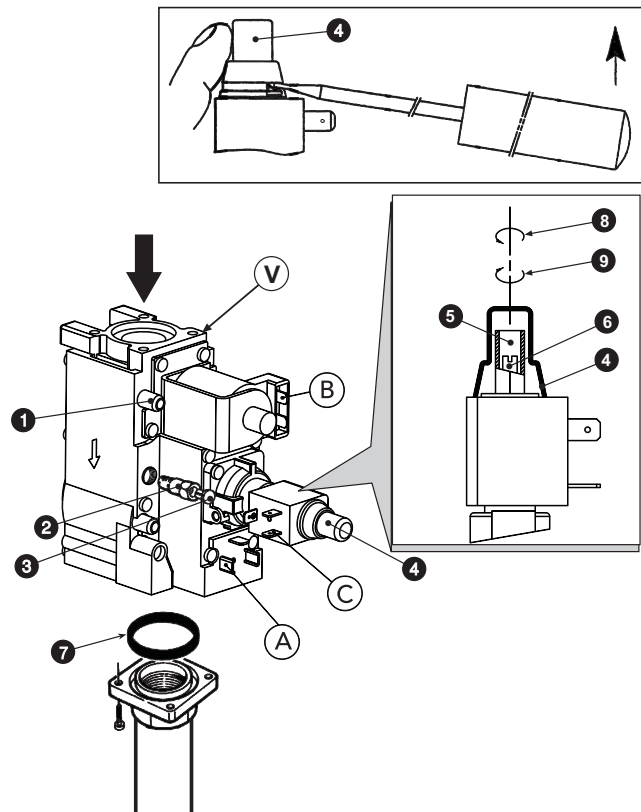
fig. 4 - Gas conversion
