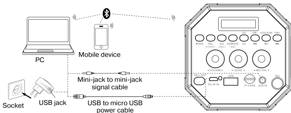
Fig. 2. Connection diagram
