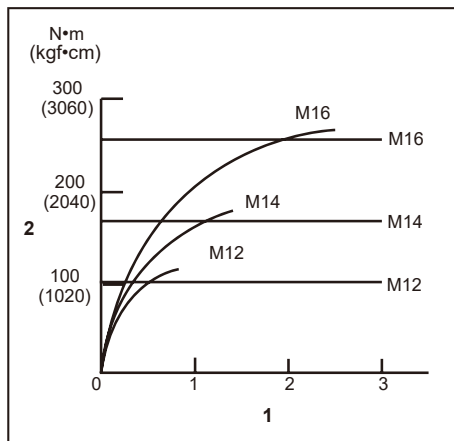
1. Fastening time (second) 2. Fastening torque
