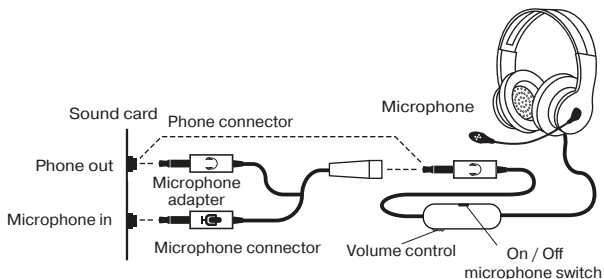
Fig. 1. Connection diagram
