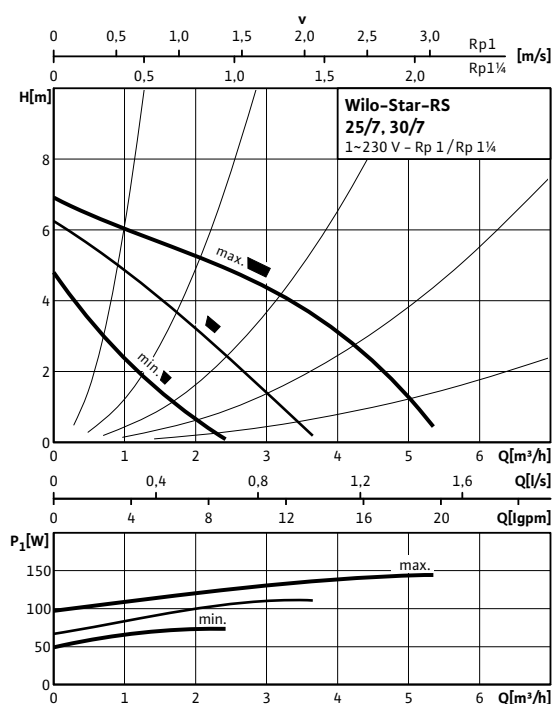
Wilo-Star-RS 25/7 - 30/7
